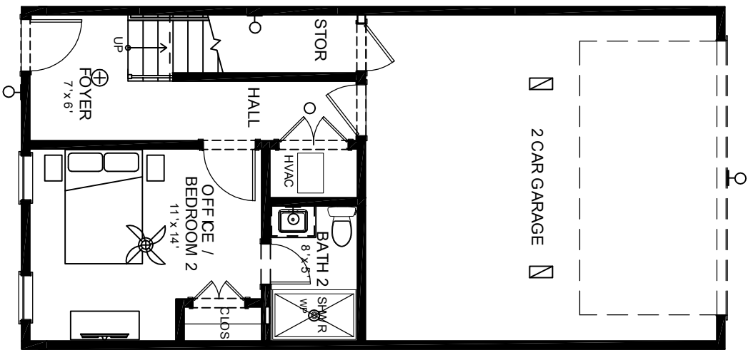
UNIT A-3 - FIRST FLOOR EXTERIOR - WHITE INTERIOR - SCHEME 1
