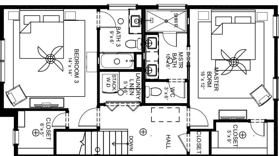
UNIT A-1 THIRD FLOOR
