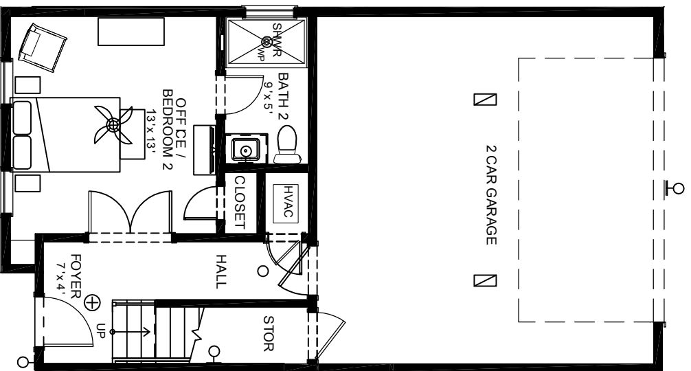
UNIT A-1 - FIRST FLOOR EXTER DR - WHITE INTER DR - SCHEME 1
